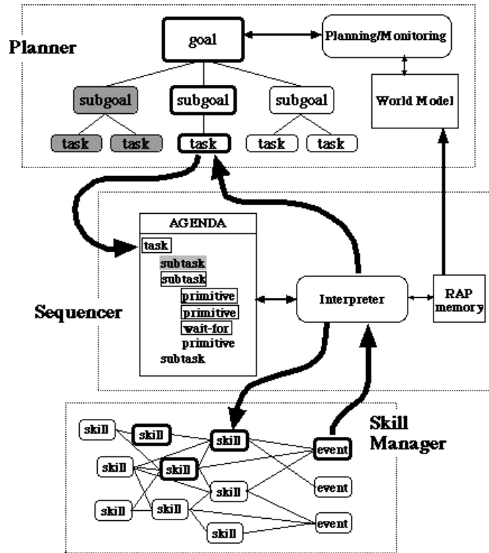
Figure 5. 3T architecture
