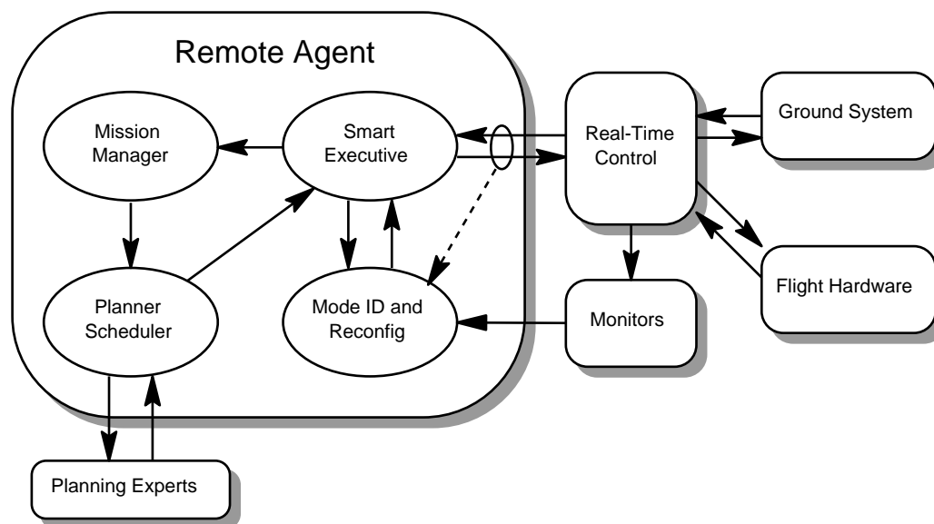
Figure 2. Remote Agent architecture
