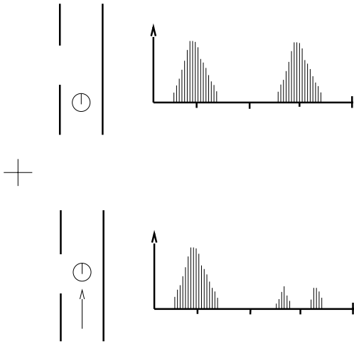
Figure 5: Detecting region boundaries using VFH.
